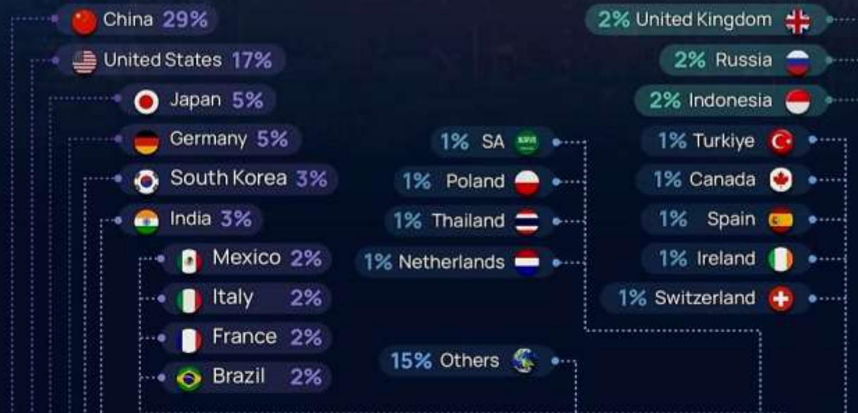
Share of global manufacturing value in 2023
